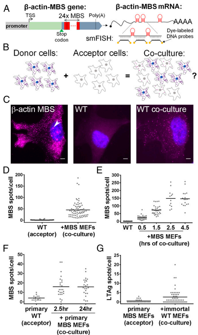
Fig. 1. Detection of \beta -actin–MBS mRNA transfer by smFISH. ( A ) A schematic depicting the \beta -actin–MBS gene ( Left ) and resulting mRNA ( Right ). mRNA detection was accomplished using smFISH with fluorescence-labeled DNA probes against the MBS sequence (aka “MBS probes”). Poly(A), polyadenylation site; TSS, transcription start site. ( B ) A schematic illustrating the basic experimental set-up. Donor cells ( Left ) that express a unique mRNA (e.g., \beta -actin–MBS; shown as small purple dots) were cocultured with naive acceptor cells ( Middle ) that lack this mRNA. If mRNAs undergo transfer from donor to acceptor cells, coculture yields labeling of the acceptor cells ( Right ). Each cell type was also cultured separately to assess mRNA-expression levels in donor cells or background staining in acceptor cells. ( C ) smFISH images of an immortalized donor MBS MEF, immortalized acceptor WT MEF, and acceptor WT MEF in coculture. Labels: blue, DAPI staining of the nucleus; magenta, Cy3-tagged MBS probes. The arrowhead indicates a transcription site. (Scale bars: 5 \mu m.) ( D ) Distribution of the number of \beta -actin–MBS mRNA spots observed in immortalized WT MEFs (expressing low levels of GFP) cultured alone or cocultured with donor MBS MEFs for 24 h. Each dot in D – G represents the score of the number of mRNAs detected in a single cell as obtained by smFISH. The horizontal bars in D – G indicate mean number of spots per acceptor cell. ( E ) Distribution of the number of \beta -actin–MBS mRNA spots in WT MEFs as a function of time after coculture with donor MBS MEFs. ( F ) Distribution of the number of \beta -actin–MBS mRNA spots in primary WT MEFs cultured alone or cocultured for 2.5 or 24 h with primary donor MBS MEFs. ( G ) Distribution of the number of LTag mRNA spots in primary MBS MEFs cocultured with LTag-immortalized donor WT MEFs for 24 h. See Dataset S1 for data on the number of cells scored, mean, SEM, and P values for each experiment.
