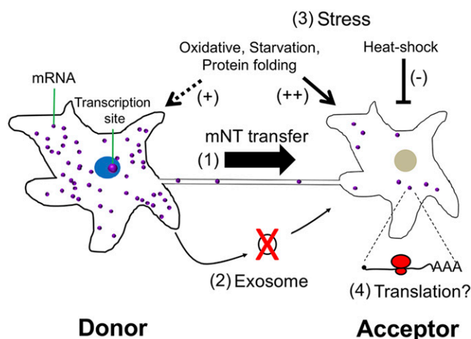
Fig. 6. A schematic representation of intercellular mRNA transfer. (1) A donor cell (Left) that expresses a given mRNA can transfer mRNA molecules to an acceptor cell (Right) through a mNT. (2) This process appears to be actin-myosin regulated, requires direct physical contact, and does not occur via exosomes. (3) Stress conditions appear to affect mRNA transfer, whereby oxidative, protein-folding, and nutrient stresses on both donor and acceptor cells favor transfer, whereas heat shock of acceptor cells inhibits transfer. (4) Transferred mRNAs are likely to undergo translation, although this has not yet been proven.
