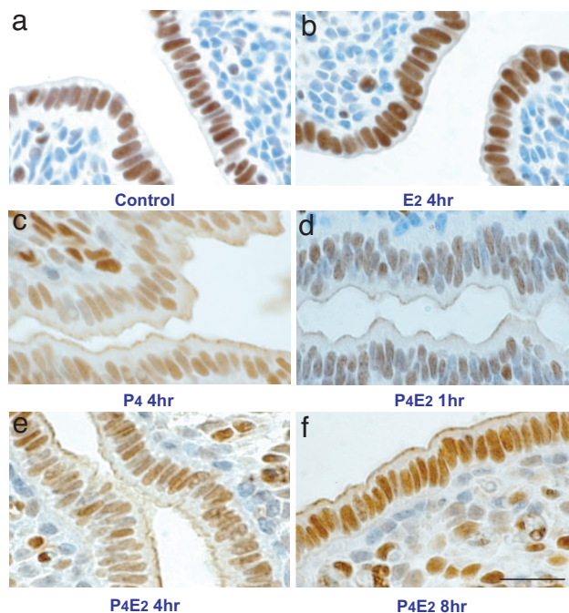
Fig. 3. P_4 transiently excludes MCM6 from the nucleus. Shown is immunostaining for MCM6 of uterine transverse sections isolated at the indicated times after the different hormonal treatments. (a) Control. (b) Fifty nanograms of E_2 at 4 h. (c) One milligram of P_4 for 4 days. (d–f) One milligram of P_4 for 4 days and killed 1 h (d), 4 h (e), and 8 h (f) after 50 ng of E_2 on the fourth day. (Scale bar: 50 \mu\text{m} .)
