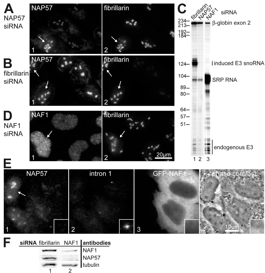
Figure 6. NAP57 and NAF1 RNA interference. (A) Double immunofluorescence of NAP57 (panel 1) and fibrillarin (panel 2) in E3 cells 3 d after transfection with NAP57 siRNA. Note that NAP57 is not knocked down in all cells (arrow). (B) Same as A, except the cells were transfected with fibrillarin siRNA. (C) RNase protection assay as in Fig. 3 E on RNA from E3 cells transfected with siRNAs directed against the mRNAs of the proteins indicated on top and induced for transgene expression. Note that NAP57 and NAF1, but not fibrillarin, siRNAs abolished specifically the accumulation of induced rat E3 snoRNA but not of the exon of the gene from which it was expressed. (D) Same as A, except the cells were transfected with NAF1 siRNA. (E) NAF1 is not present at the H/ACA RNA transcription site in cells knocked down for NAP57. Triple fluorescence of endogenous NAP57 (panel 1), FISH with intron 1 probe marking the transcription site (panel 2), and transfected GFP-NAF1 (panel 3) in cells transfected with NAP57 siRNA. Panel 4 shows a phase-contrast image of the same cells and outlines the area of the inset. The arrow points to an unsilenced cell. The width of inset is 2.6 \mu m. (F) Western blots of lysates from cells treated with siRNA to fibrillarin (lane 1) and NAF1 (lane 2), probed with antibodies to the antigens indicated on the right, and scanned on an infrared imaging system.
